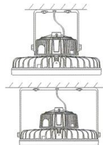
U-shaped bracket installation
