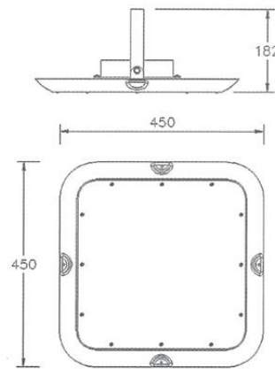
Type C U-Bracket Surface Mounted Power range:40-150W
