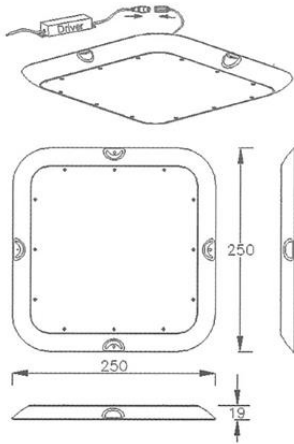
Type A Ceiling Mounted Power:30W
