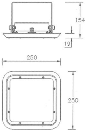
Type B U-Bracket Surface Mounted Power:30W
