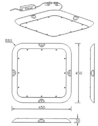
Type D Ceiling Mounted Power range:40-150W
